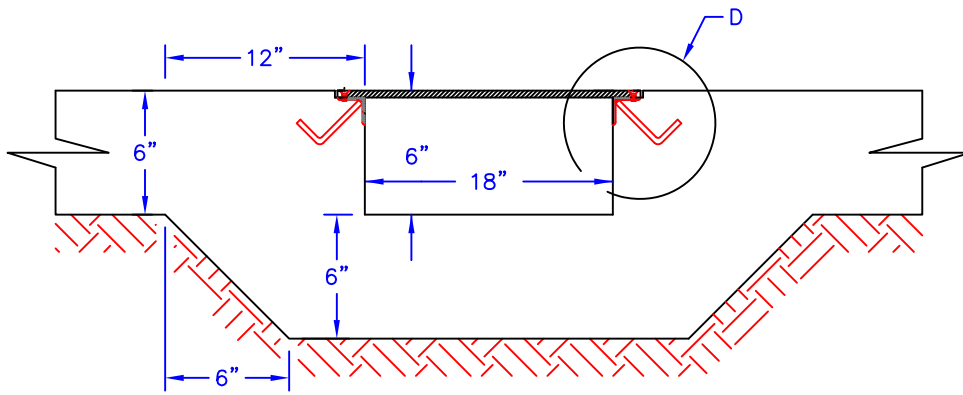
CHASE SECTION (TYP.)
